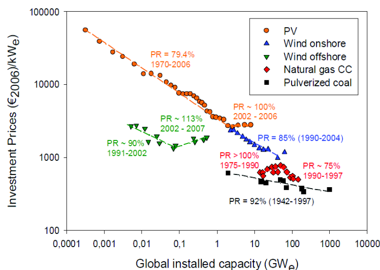
FIGURE C-2 Comparison of historical experience curves and progress ratios ( PR = 1 - \text{learning rate} ) of energy supply technologies. SOURCE: Junginger et al., 2008, p. 10.
