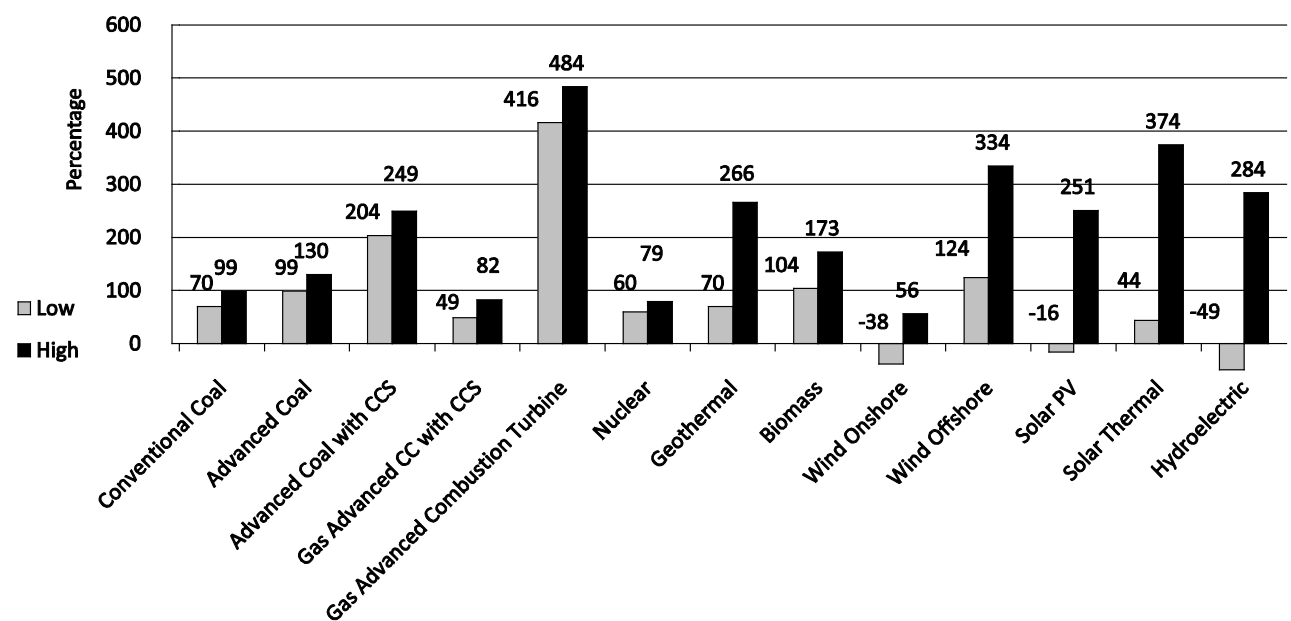
FIGURE 2-8 Percent difference in levelized cost of electricity (LCOE) estimates for electric power generation technologies entering the market in 2020 compared with conventional combined-cycle natural gas power generation when pollution costs are externalized. NOTE: CC = combined cycle; CCS = carbon capture and storage; IGCC = integrated gasification combined cycle; PV = photovoltaic. SOURCE: Sullivan et al., 2015.
